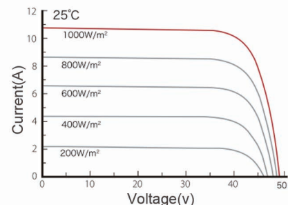
Current-voltage(570W)
